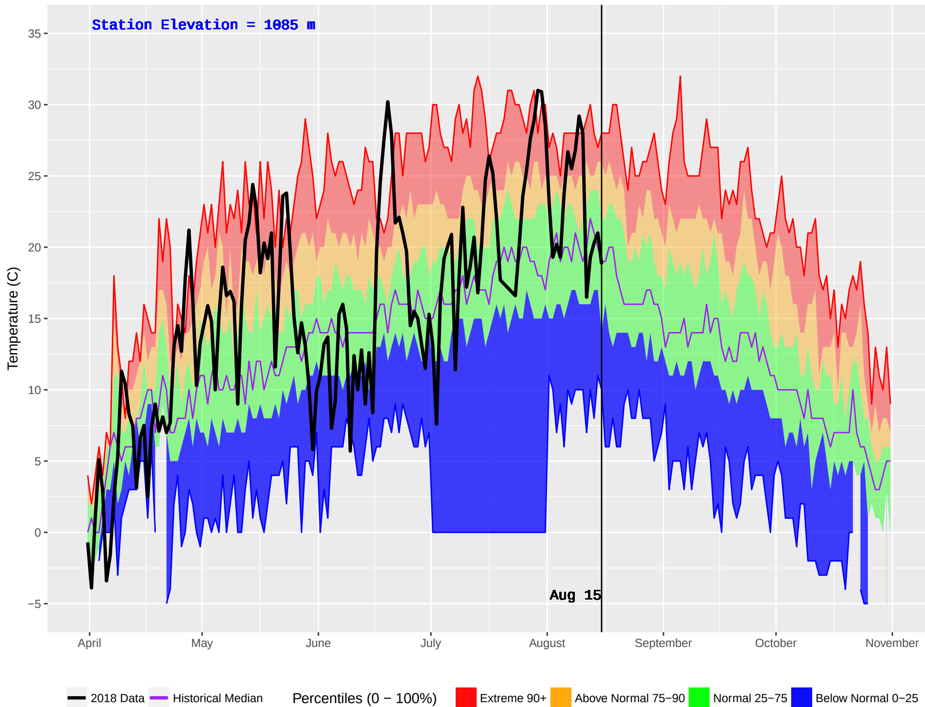
TAUTRI (206) : Historical (1970–2016) and Current (2018) Daily Temperature
