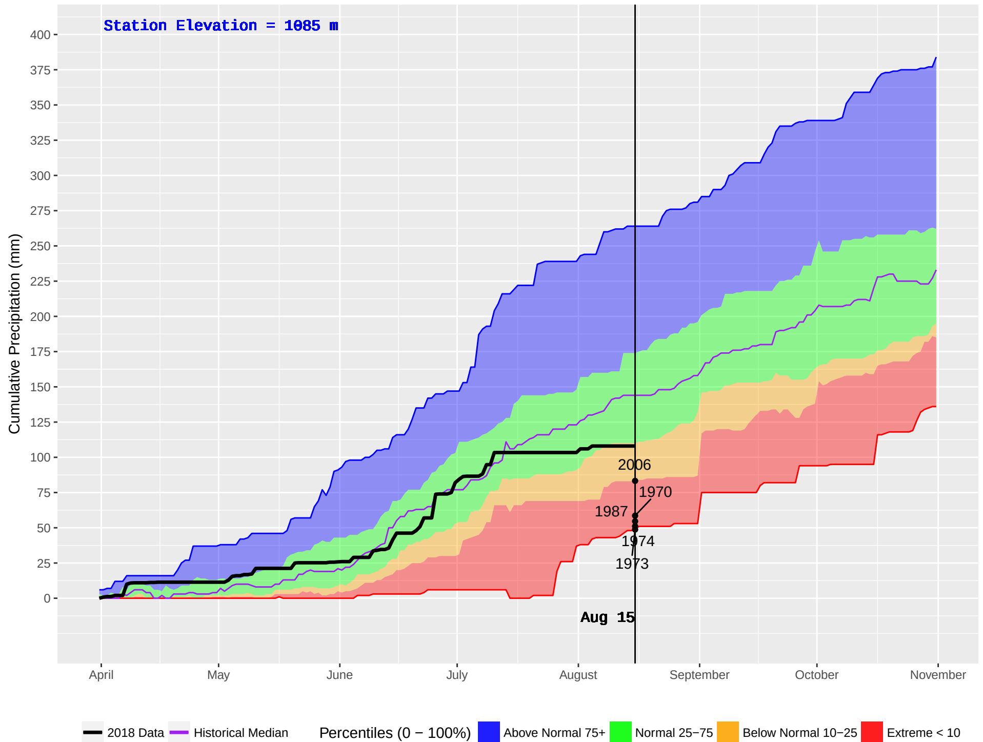
TAUTRI (206) : Historical (1970–2016) and Current (2018) Daily Cumulative Precipitation
