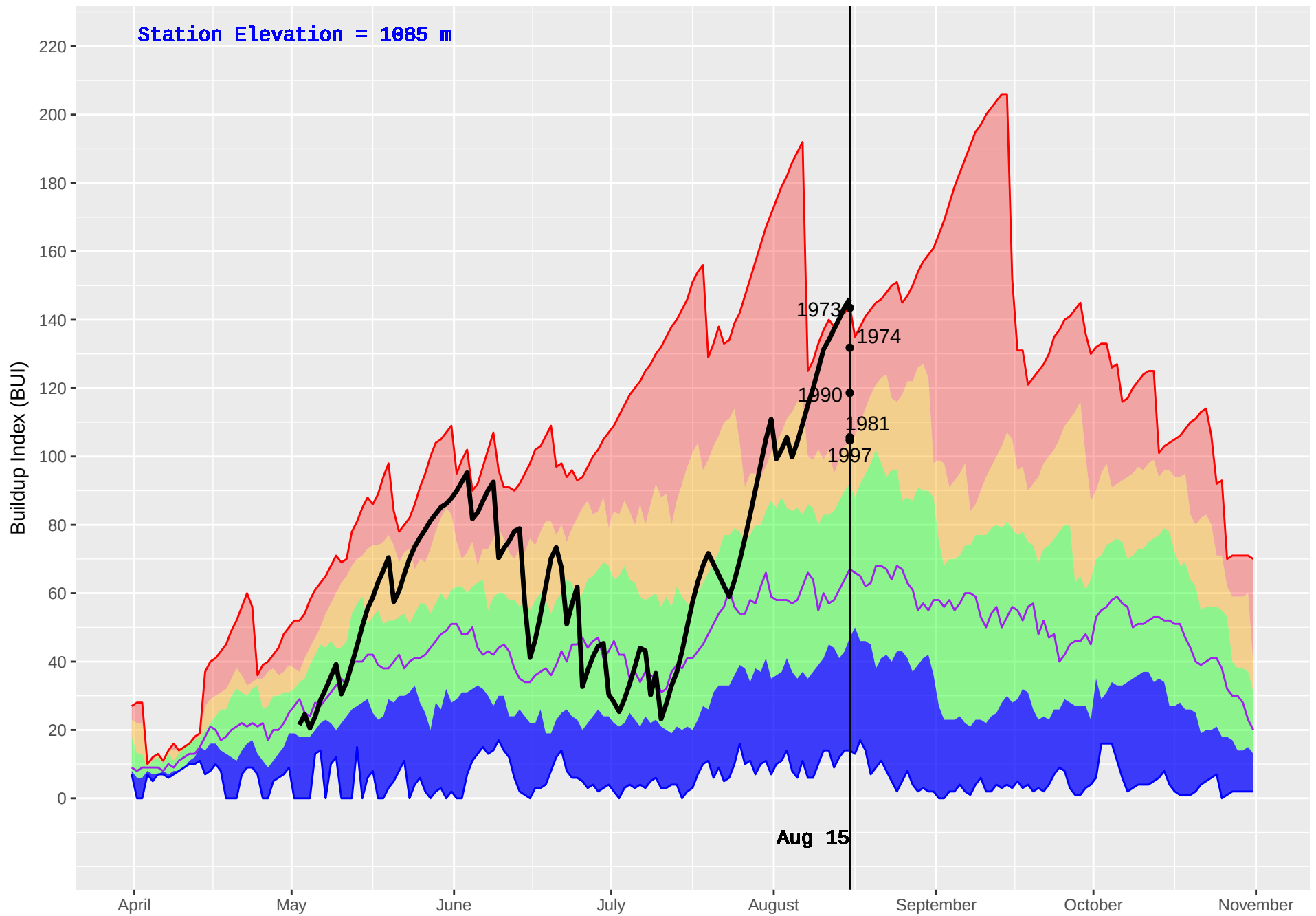
TAUTRI (206) : Historical (1970–2016) and Current (2018) Daily Buildup Index (BUI)
